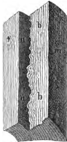
Fig. 58.—(a a) Surface peeled by deer. (b b) Wood occluding the wound and subsequent layers.
